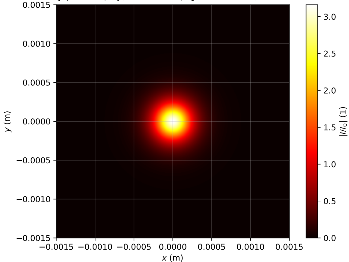
Intensity profile I(x, y, z = 3.742\text{m})/I_0 , Pin=1.0Pcr, artificial time
